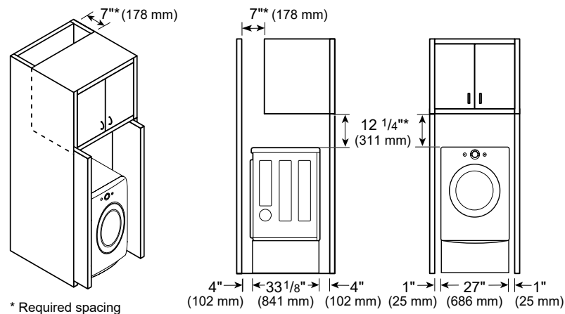
Closet installation with pedestal
